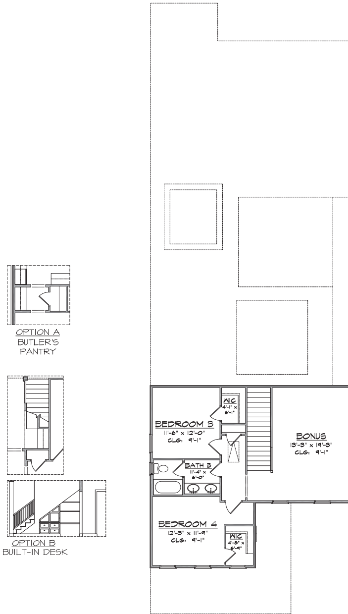
UPPER LEVEL FLOOR PLAN
