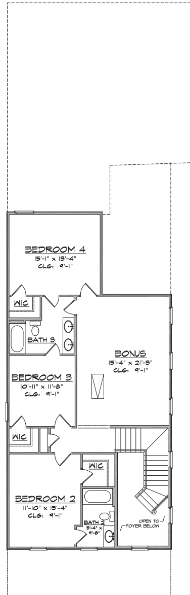
UPPER LEVEL FLOOR PLAN
