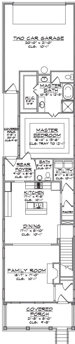
MAIN LEVEL FLOOR PLAN
