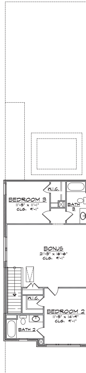
UPPER LEVEL FLOOR PLAN
